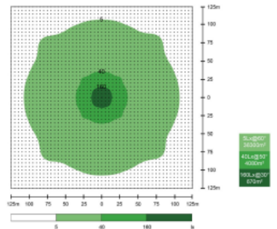
Without Diffuser
