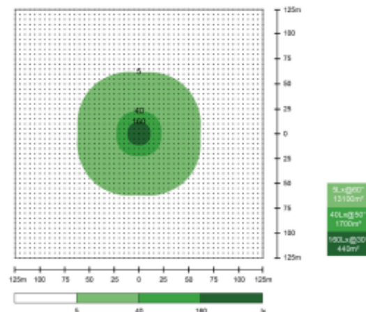
With Diffuser
