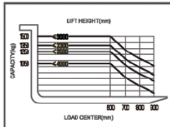
LOAD CHART
