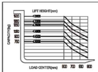
LOAD CHART
