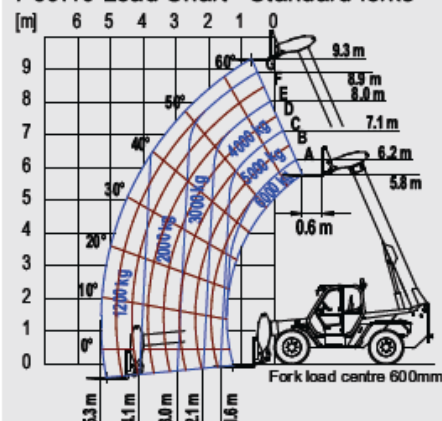
P60.10 Load Chart - Standard forks
