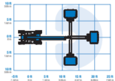
Jib range of motion Z-30/20N RJ
