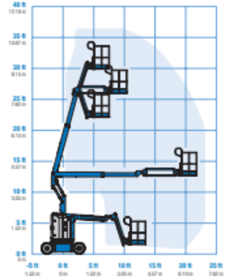
Jib range of motion Z-30/20N RJ
