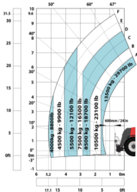
MHT 10135 ST5 - Load chart
