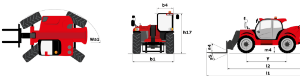
MHT 10135 ST5 - Dimensional drawing
