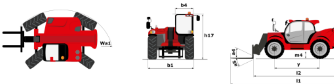
MHT 10135 ST5 - Dimensional drawing
