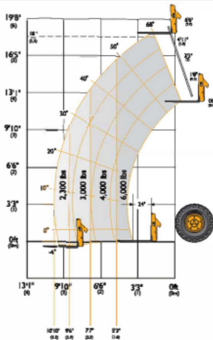
LIFT PERFORMANCE – 527-55
