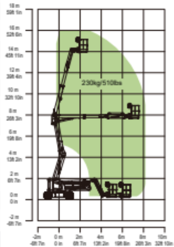
Range of Motion ZA14NJE
