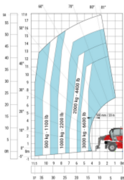
Machine on tyres with forks Metric
