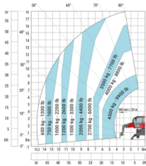
Machine on lowered stabilisers with forks Metric
